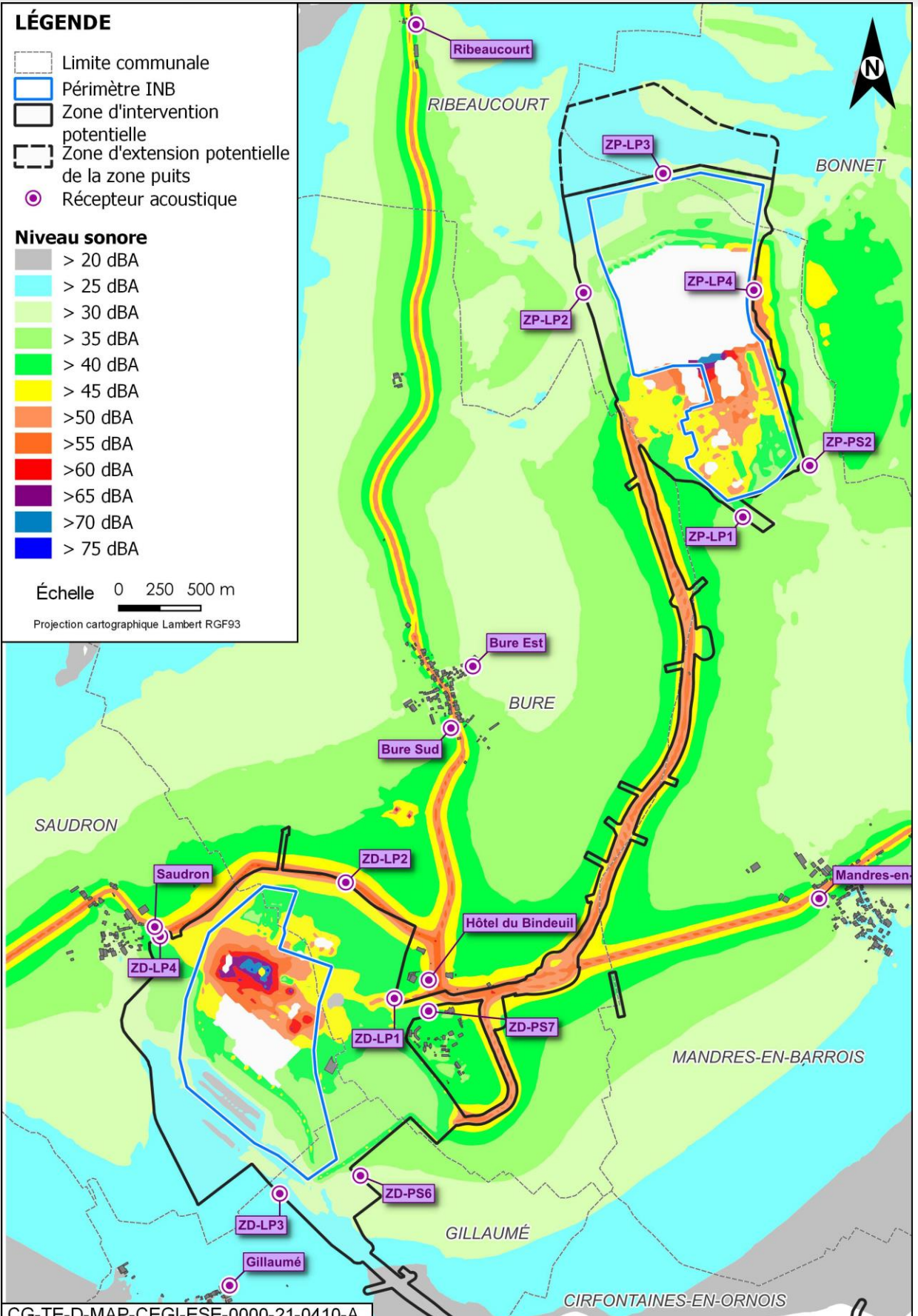
Figure 2-5 Propagation acoustique - Construction initiale - Toutes sources (nocturne)
